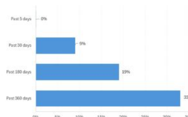
PB ratio
