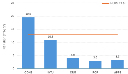
PB ratios
