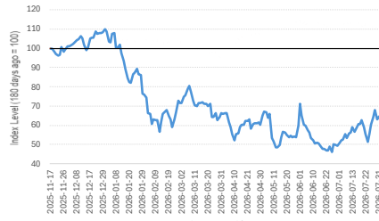
HUBS vs S&P 500 (180 days)
