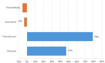
PB ratios
